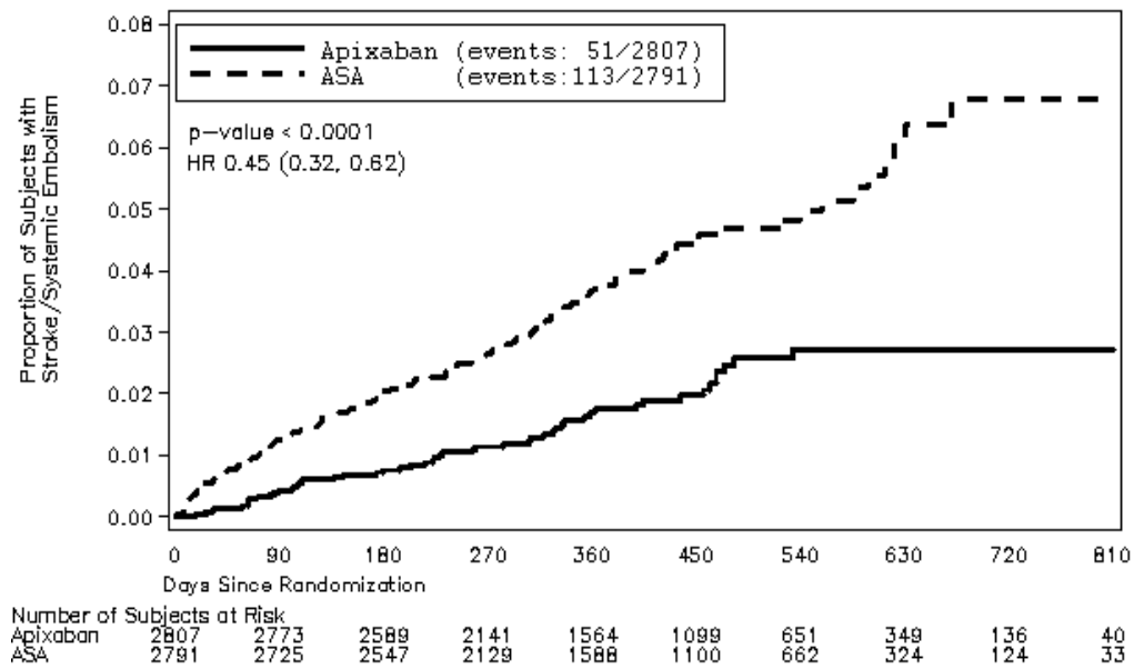
Figure 2 - Kaplan-Meier Curve Estimate of Time to First Occurrence of Stroke or Systemic Embolism in the AVERROES Study
